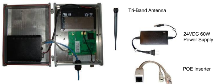
EZ-Base™ Interior View
