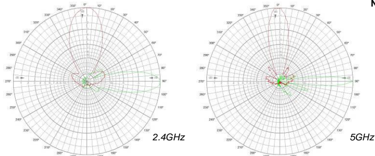
EZ-Bridge-LT™ Antenna Patterns
